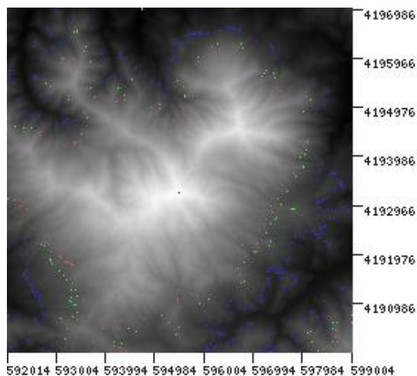
Z:10 E: 592014 N: 4189996 Map of Mt. Diablo, California, UTM imager module, C5 Landscape database (2002)
